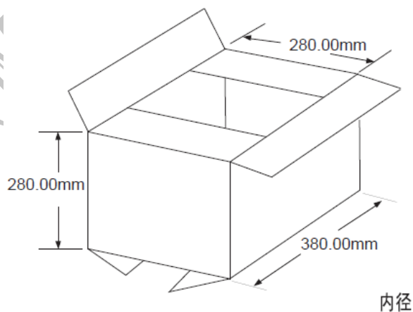
Figure 50: Big carton drawing
