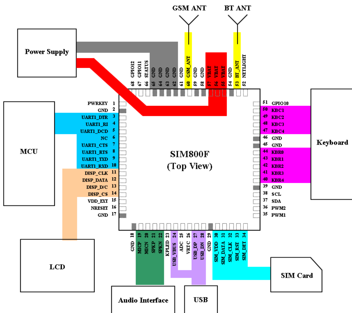
Figure 44: Pin assignment
