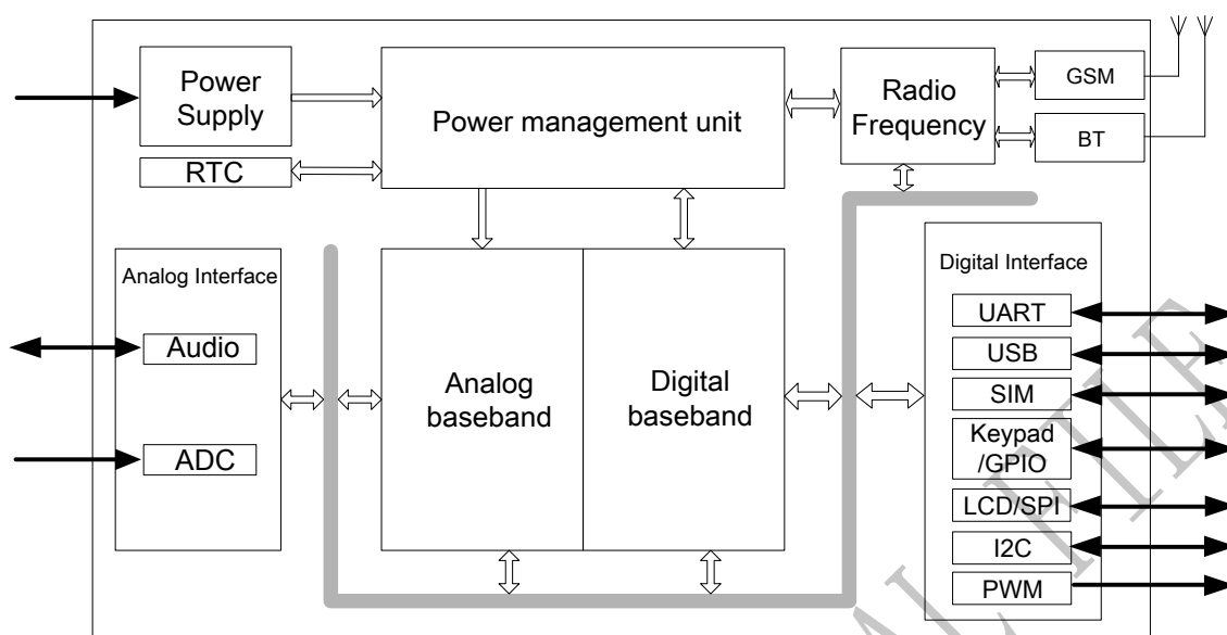
Figure 1: SIM800F functional diagram
