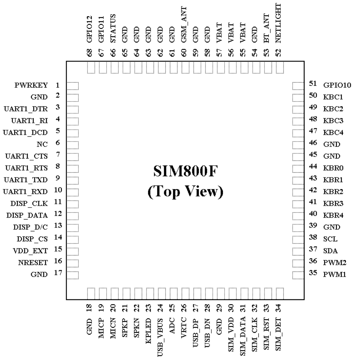
Figure 2: SIM800F pin out diagram (Top view)
