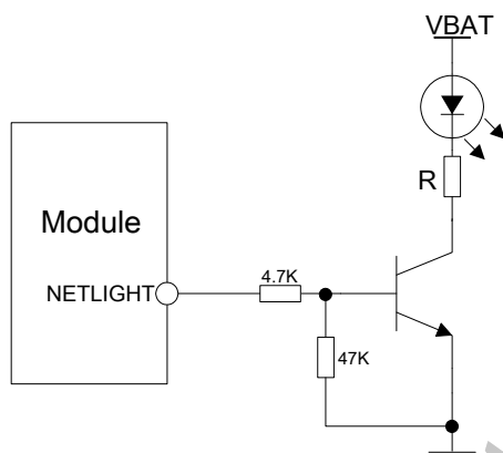
Figure 38: Reference circuit of NETLIGHT
