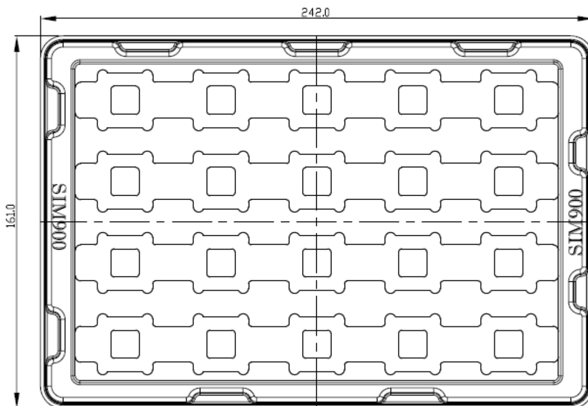
Figure 48: Module tray drawing
